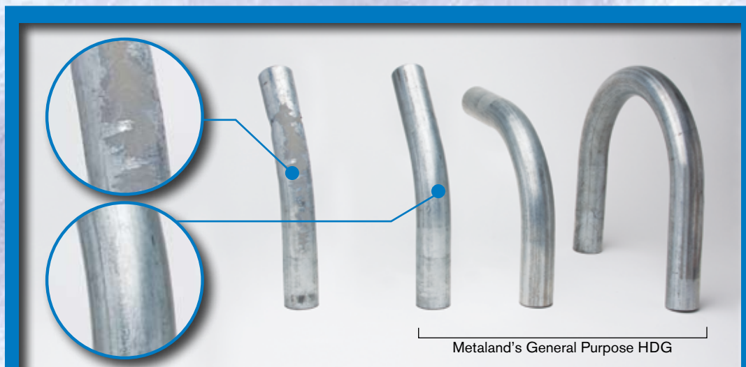
Some galvanized pipe can flake when bending (far left). Thanks to its high quality Hot Dipped Galvanized coating, Metaland's General Purpose HDG resists flaking even when bent 180 degrees*.
